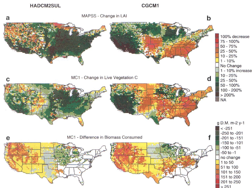
Figure 12. (a), (b) Simulated percentage change in LAI (MAPSS model at 0.5° latitude/longitude resolution) vs (c, d) change in live vegetation carbon (MC1) under HADCM2SUL and CGCM1 scenarios. MAPSS results are the change between the 2070–99 period and the baseline historical period. MC1 results compare average vegetation carbon of the last decade of the century to that of the 1961–90 period. (e, f) Absolute change in average annual biomass consumed as simulated by MC1, comparing the long-term average for the entire historical period (1895–1993) to that of the entire future climate change period (1994–2099) under HADCM2SUL and CGCM1.
