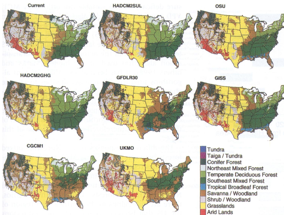
Figure 3. MAPSS-simulated vegetation distribution for the conterminous US (10-km resolution) under the seven GCM climate scenarios listed in Figure 1.
