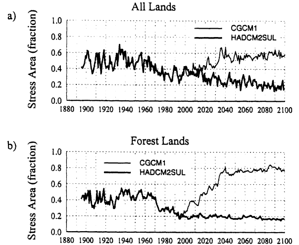
Figure 14. MCI-simulated stress area under historical climate and future climate scenarios for (a) the conterminous US and (b) forested lands only. The stress area is the area of the US or of the US forest lands where live vegetation C density is less than that of the long-term average carbon density calculated for the 100-year spin-up period.
