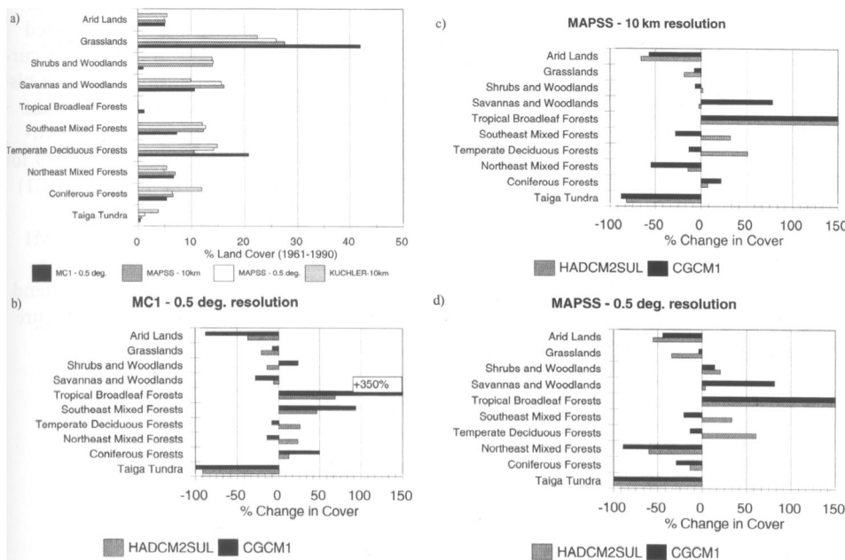
Figure 5. (a) Percentage land cover of simplified potential vegetation types simulated by MC1 (1990) and MAPSS (baseline historical climate) over the conterminous US compared to Küchler's (1975) potential vegetation map. (b) Percentage change in area of the simplified vegetation types as simulated by MC1 under two transient scenarios for the year 2095. (c) Percentage change in area of the simplified vegetation types as simulated by MAPSS at 10-km resolution under an average climate (2070–99) from the same two scenarios (since there were no tropical broadleaf forests under historical conditions, percentage change has been arbitrarily set to 150%). (d) Same as c, but for 0.5° latitude/longitude resolution.
