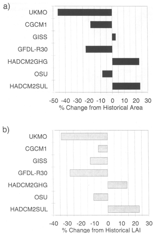
Figure 4. Percentage changes in (a) forest area and (b) forest LAI for the conterminous US between current and future conditions for the seven GCM climate scenarios listed in Figure 1.
